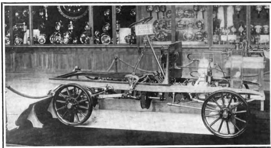
FIRST APPEARANCE OF THE FOUILLARON CAR AT AN AMERICAN SHOW—NOTE TRANSVERSE BELT TRANSMISSION BETWEEN THE STEERING PILLAR AND SIDE LEVERS.
